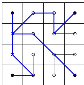
FIGURE 5. The tree T_{2,1} (in blue) for the IFS for the square in Fig. 3.
